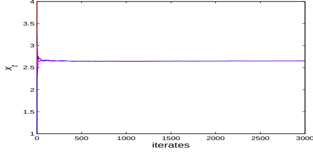
Figure 6: The 3-agent example using decreasing step size a_t = (t + 5)^{-0.85} .
