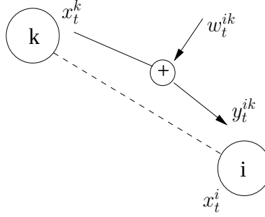
Figure 1: Measurement with additive noise w_t^{ik} .
